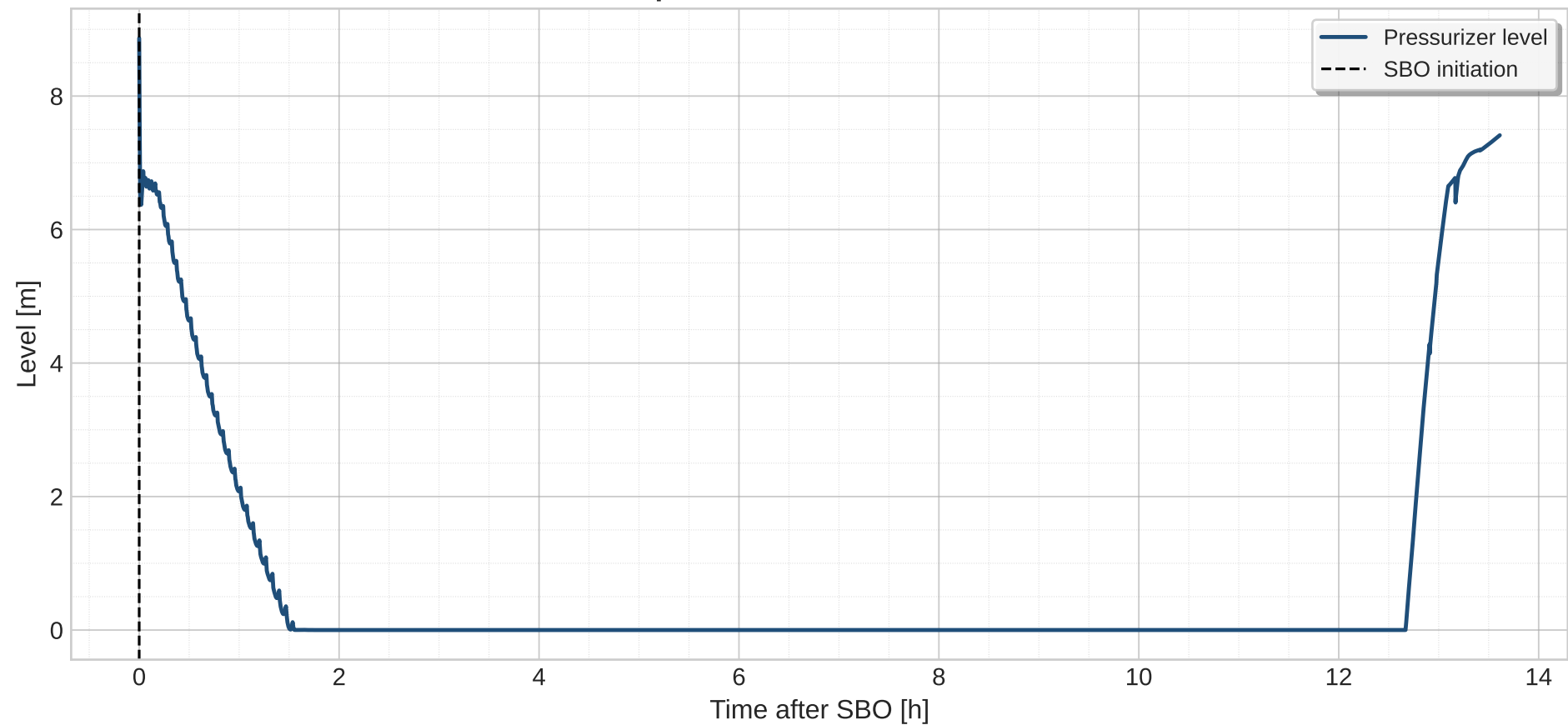
No SG Depressurization - Pressurizer Level
